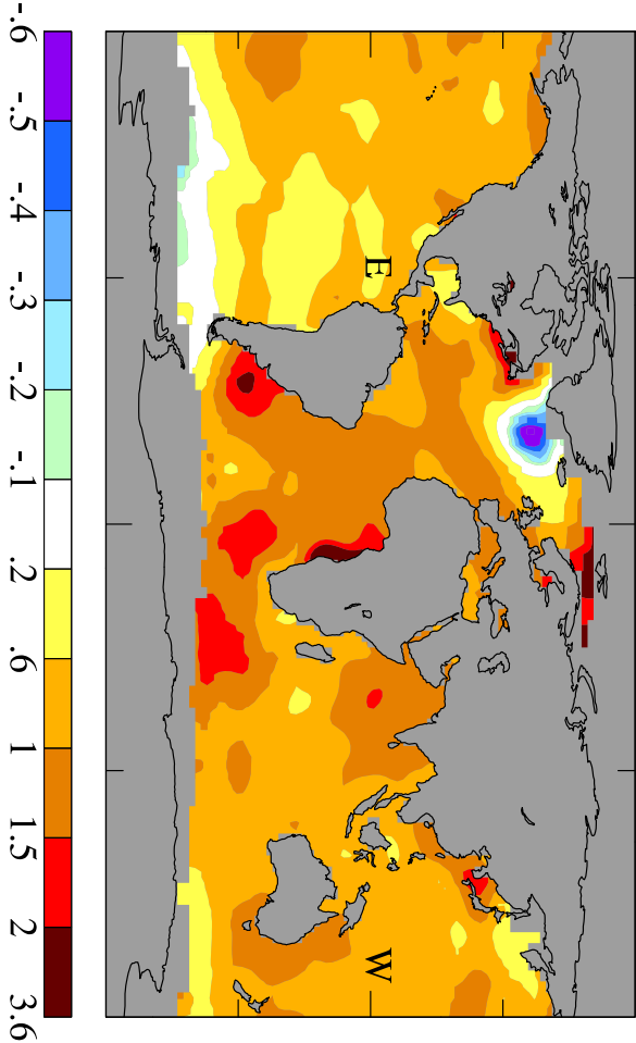
1880 to 2024 SST Change (°C) Based on Linear Trends
