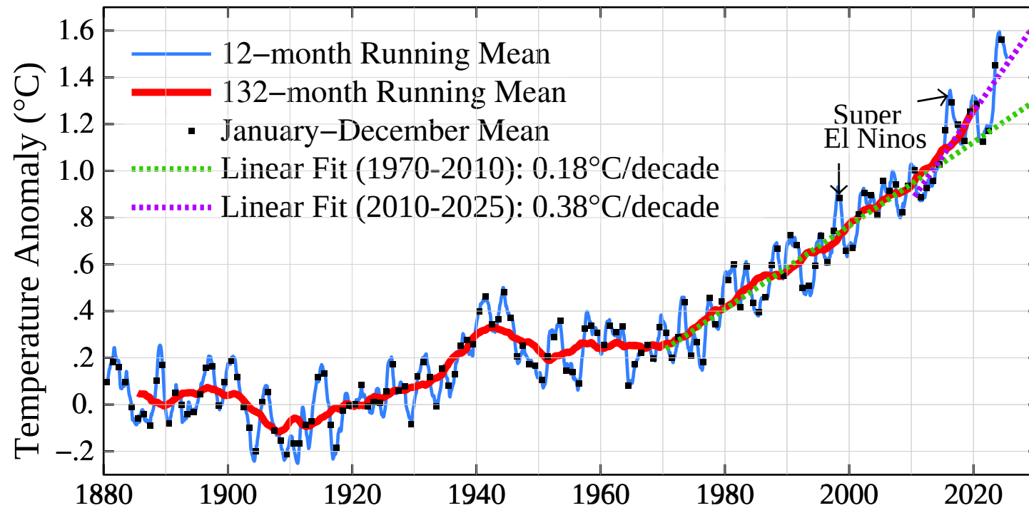
Global Surface Temperature Relative to 1880–1920 Mean
