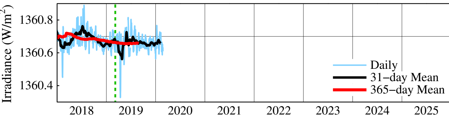
GES DISC Total Solar Irradiance
