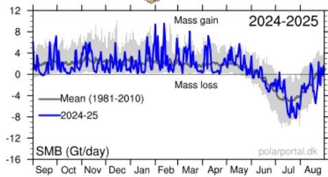
Daily
