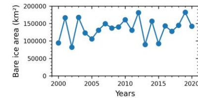
Snow lines
