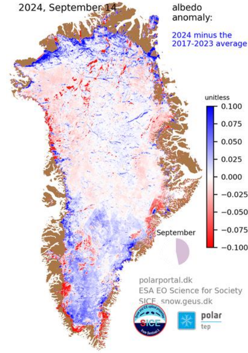
Albedo
