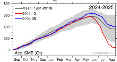
Accumulated
