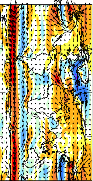
(b) Wind Speed Change (m/s)
