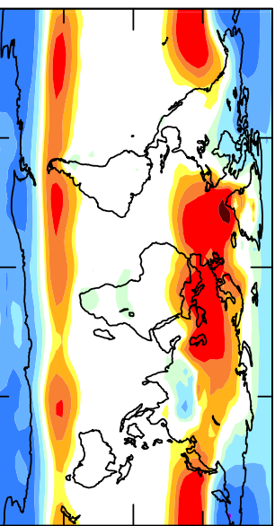
(a) Sea Level Pressure Change (hPa)
