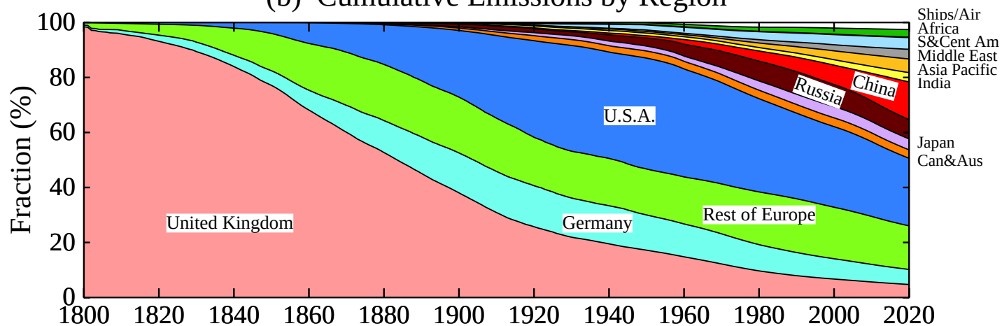
(b) Cumulative Emissions by Region
