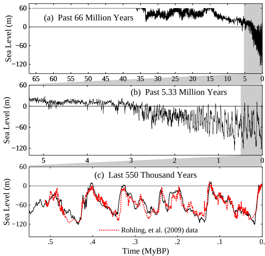
Zachos Sea Level
