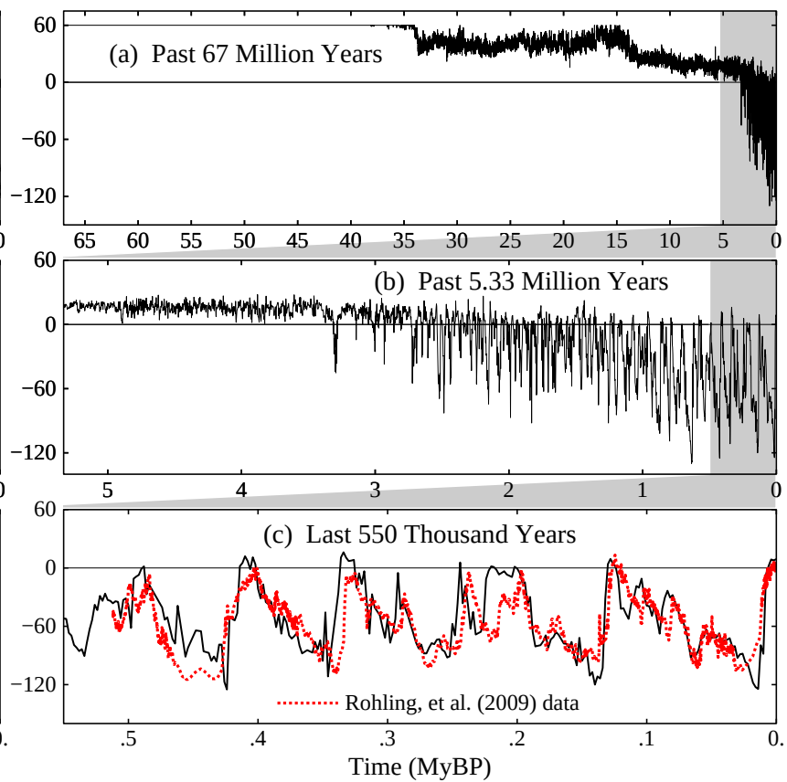
Westerhold's Sea Level
