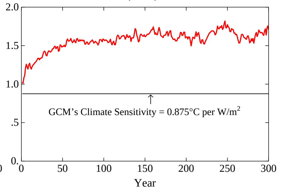
GISS (2020) Model
