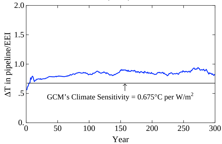
GISS (2014) Model
