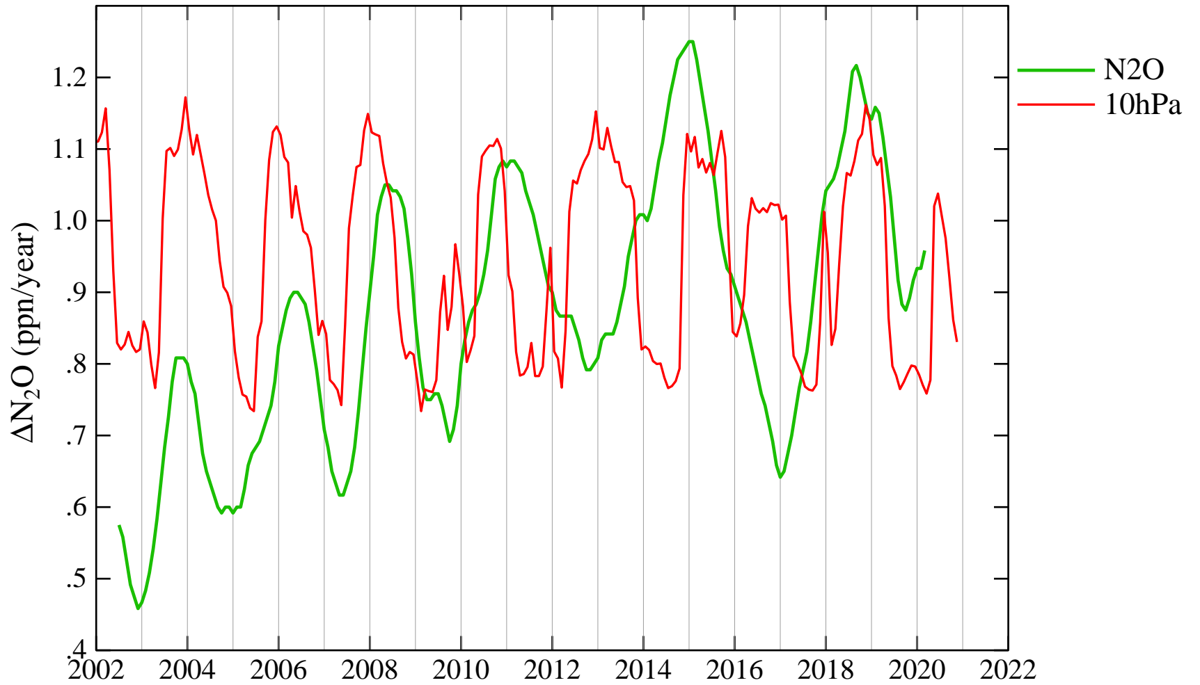
Annual Increase of Global Mean N 2 O and QBO
