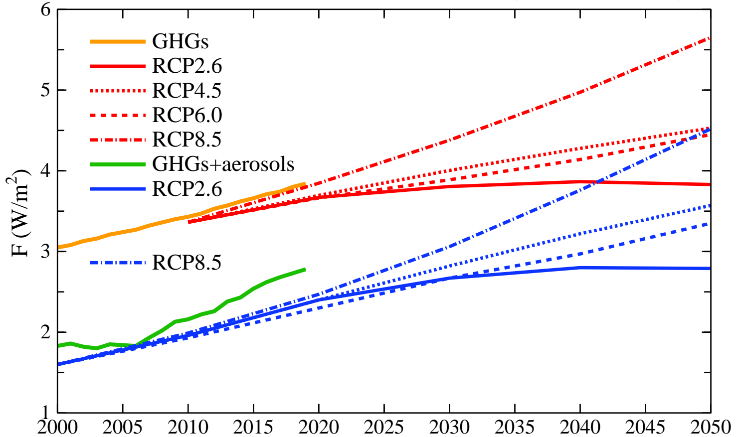
IPCC Total GHG and GHG+aerosols ERFs (Relative to 1750)
