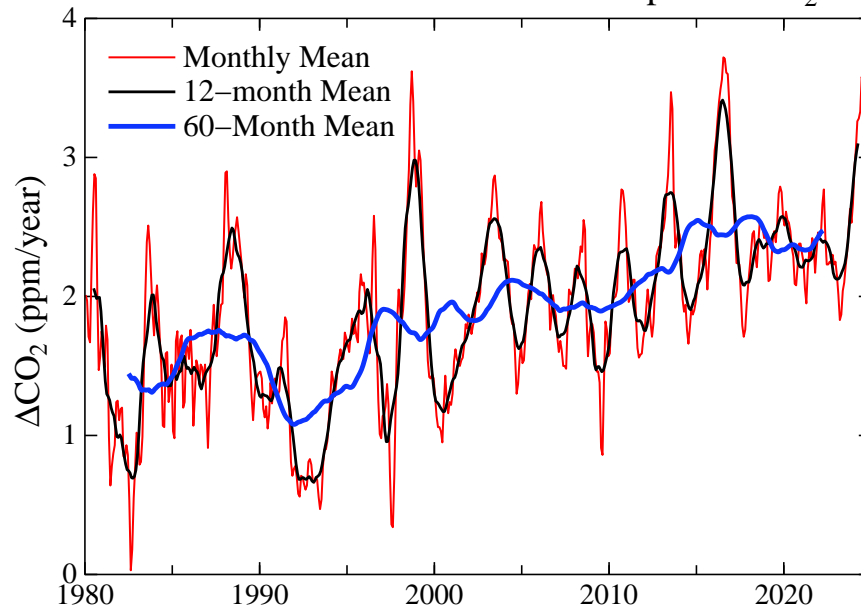
Annual Increase of Global Atmospheric CO 2
