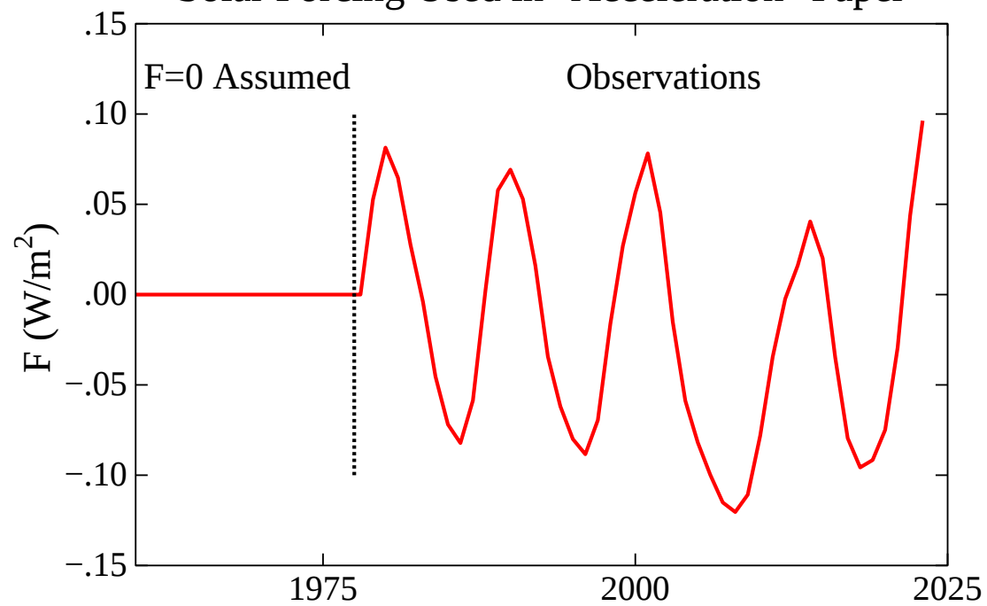
Solar Forcing Used in "Acceleration" Paper
