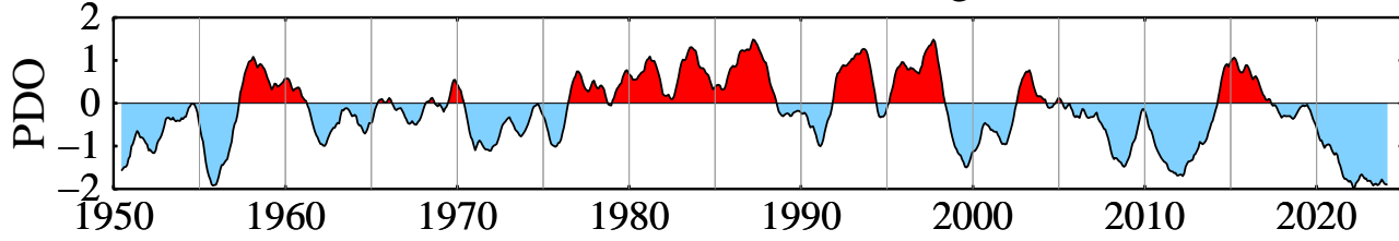
(b) PDO: 12-Month Running-Mean
