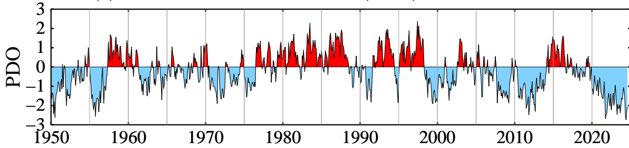
(b) PDO: 12-Month Running-Mean
