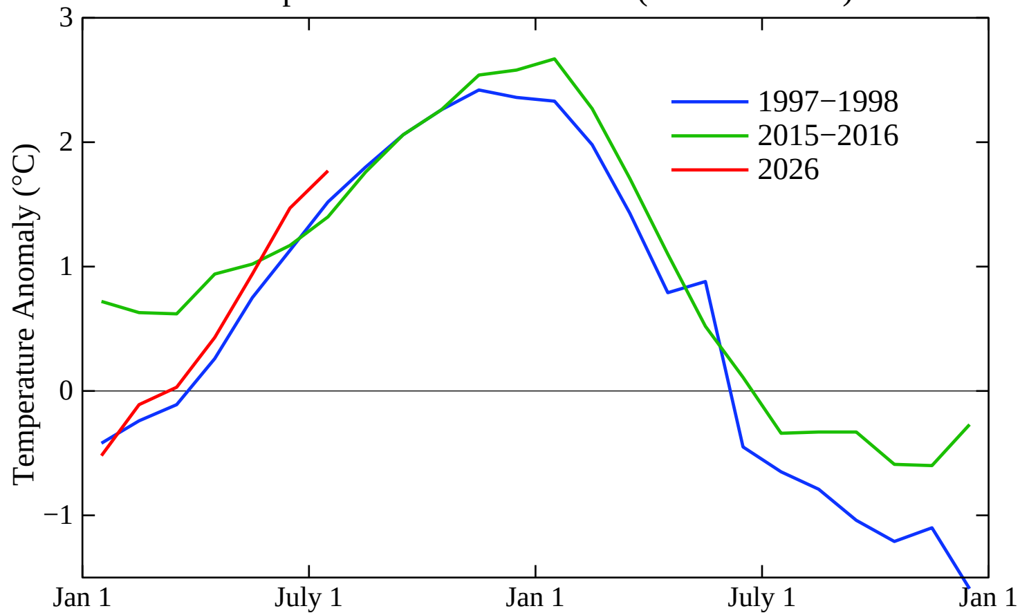
Comparison of Nino 3.4 Index (Centered Base)
