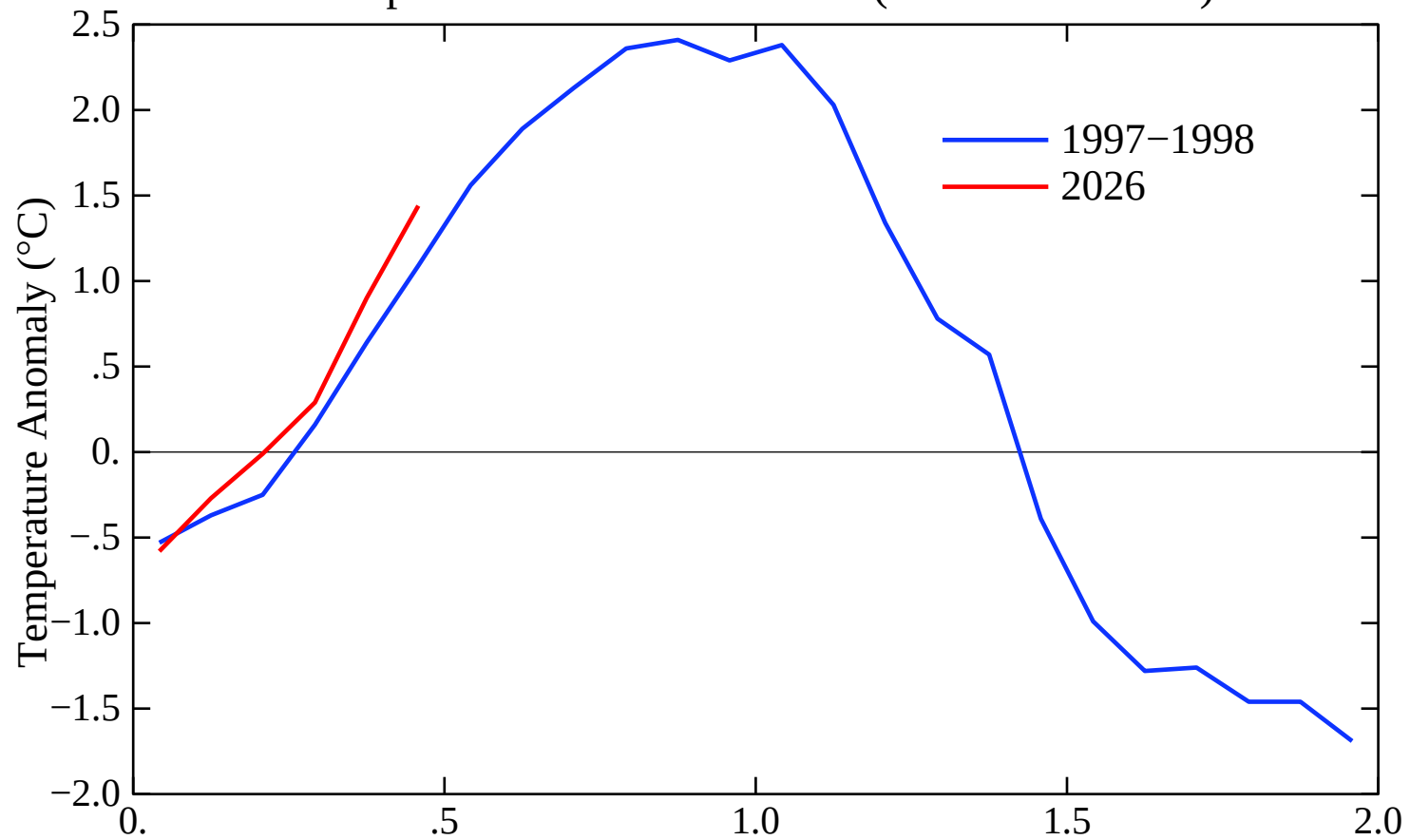
Comparison of Nino 3.4 Index (1991–2020 Base)
