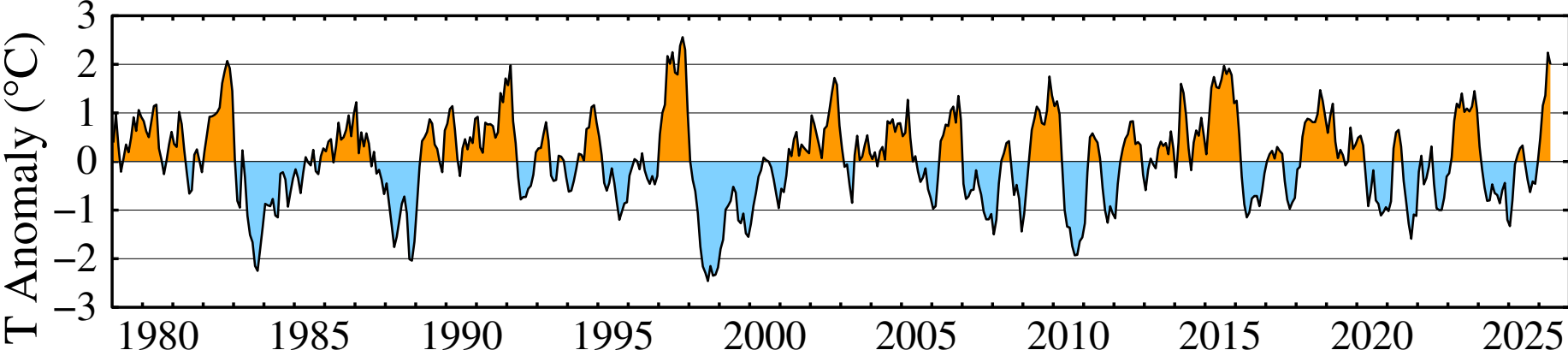
Equatorial Upper 300m T (180–100W): 1981–2010 Base
