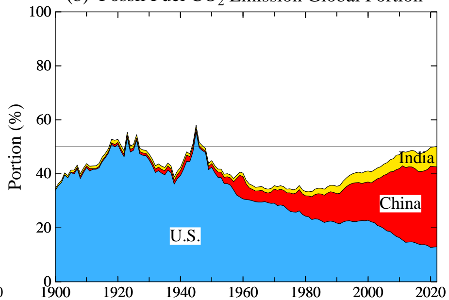
(b) Fossil Fuel CO 2 Emission Global Portion
