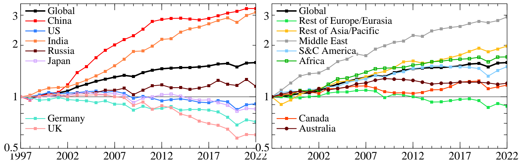
Annual CO 2 Emissions Normalized in 1997
