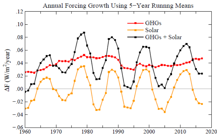
Fig. 4. Black curve is the net annual change of measured climate forcings, GHGs + Solar.
