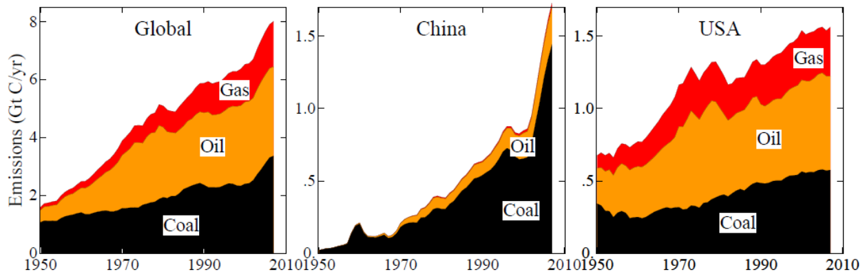
Fig. 42.1. Fossil fuel CO 2 emissions through 2007: global, China and United States.
