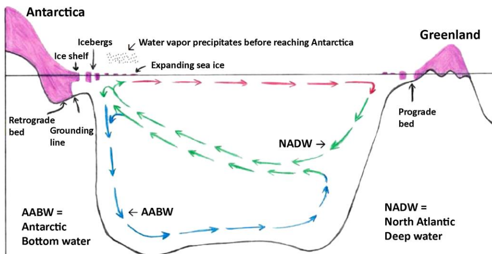
Fig. 39.2. Schematic diagram of the surface origin of two water masses that fill most of the world ocean: North Atlantic Deep Water (NADW) and Antarctic Bottom Water (AABW).
