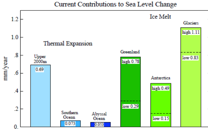
Fig.14. Estimated contributions to sea level change in 2005-2010. Upper ocean thermal expansion is from von Schuckmann and Le Traon (2011). High and low estimates for ice melt are discussed in the text.
